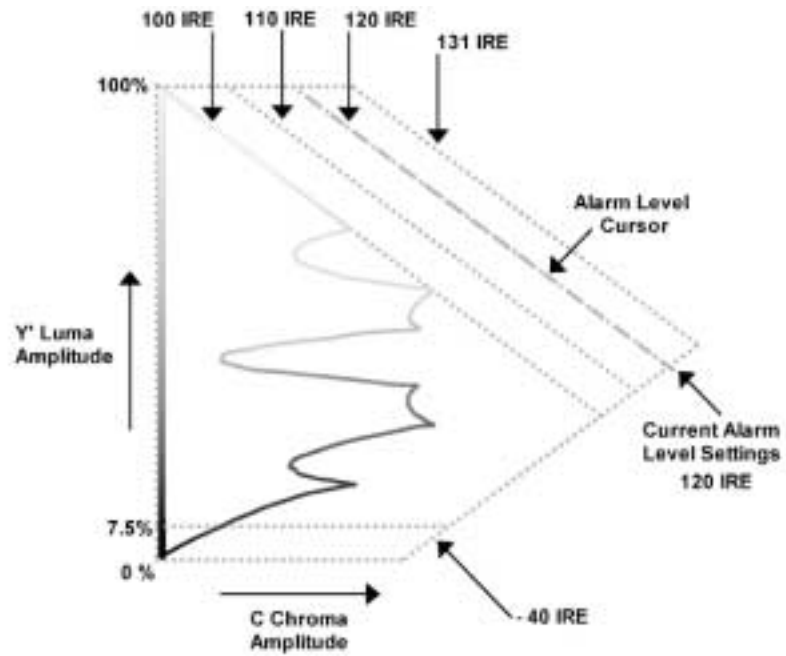
Figure 3-17: NTSC Arrowhead graticule
