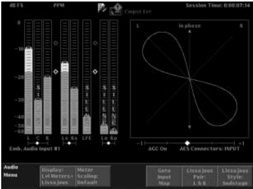
Figure 2- 6: Audio Level Meters + Lissajous display (Option DG only)
