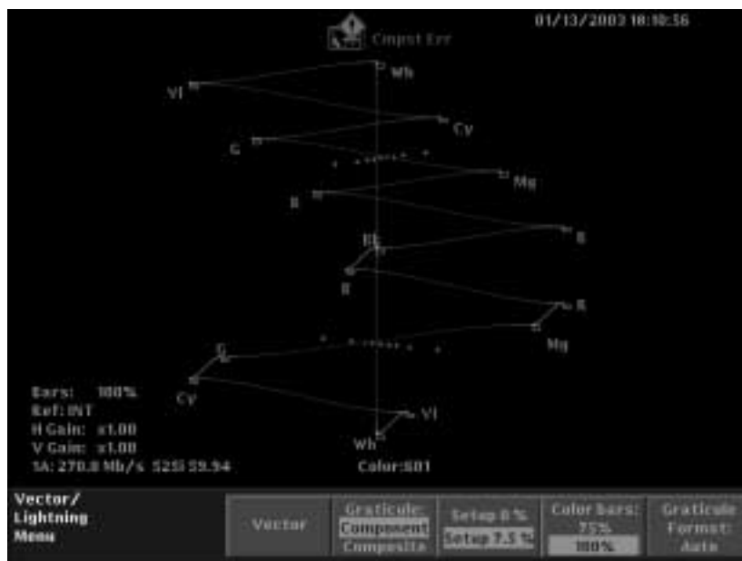
Figure 2-42: Lightning display
