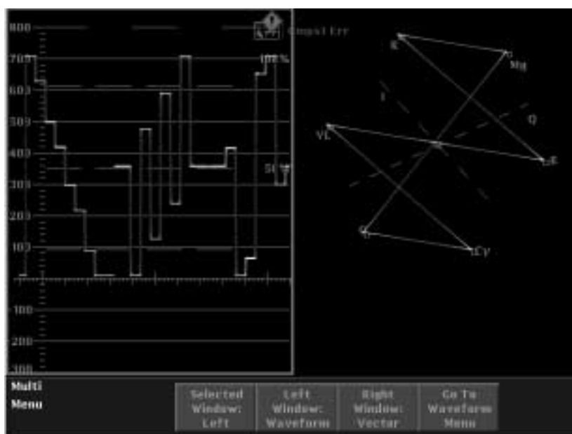
Figure 3-22: Multi mode showing the Waveform and Vector displays
