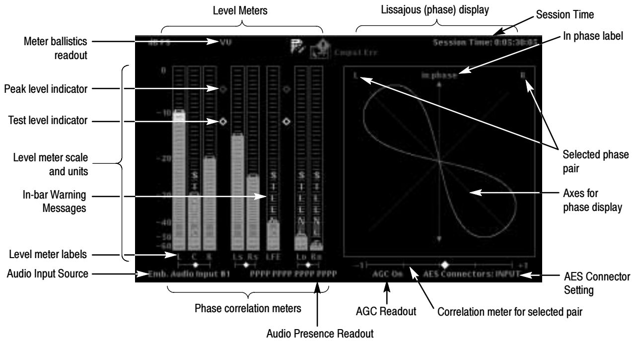
Figure 3-36: Audio Level Meters + Lissajous display
