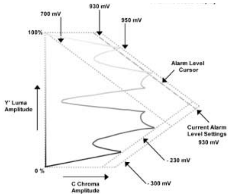
Figure 3-18: PAL Arrowhead graticule
