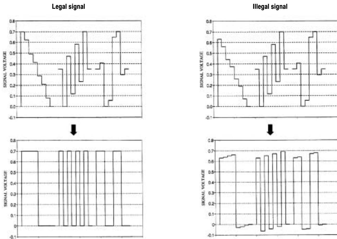
Figure 3-19: Example of legal and illegal color-difference signals
